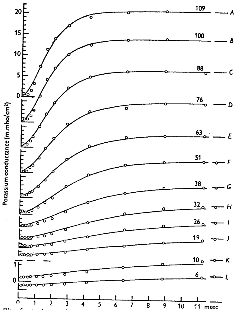
Fig. 3. Rise of potassium conductance associated with different depolarizations. The circles are experimental points obtained on axon 17, temperature 6–7° C, using observations in sea water and choline sea water (see Hodgkin & Huxley, 1952 a ). The smooth curves were drawn from eqn. (11) with g_{K0} = 0.24 m.mho/cm 2 and other parameters as shown in Table 1. The time scale applies to all records. The ordinate scale is the same in the upper ten curves (A to J) and is increased fourfold in the lower two curves (K and L). The number on each curve gives the depolarization in mV.
