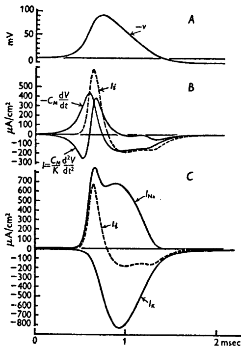
Fig. 18. Numerical solution of eqn. (31) showing components of membrane current during propagated action potential. A, membrane potential ( -V ). B, ionic current ( I_i ), capacity current ( -C_M \frac{dV}{dt} ) and total membrane current ( I = \frac{C_M}{K} \frac{d^2V}{dt^2} ). C, ionic current ( I_i ), sodium current ( I_{Na} ) and potassium current ( I_K ). The time scale applies to all the curves. Details of the analysis are as in Fig. 15.
