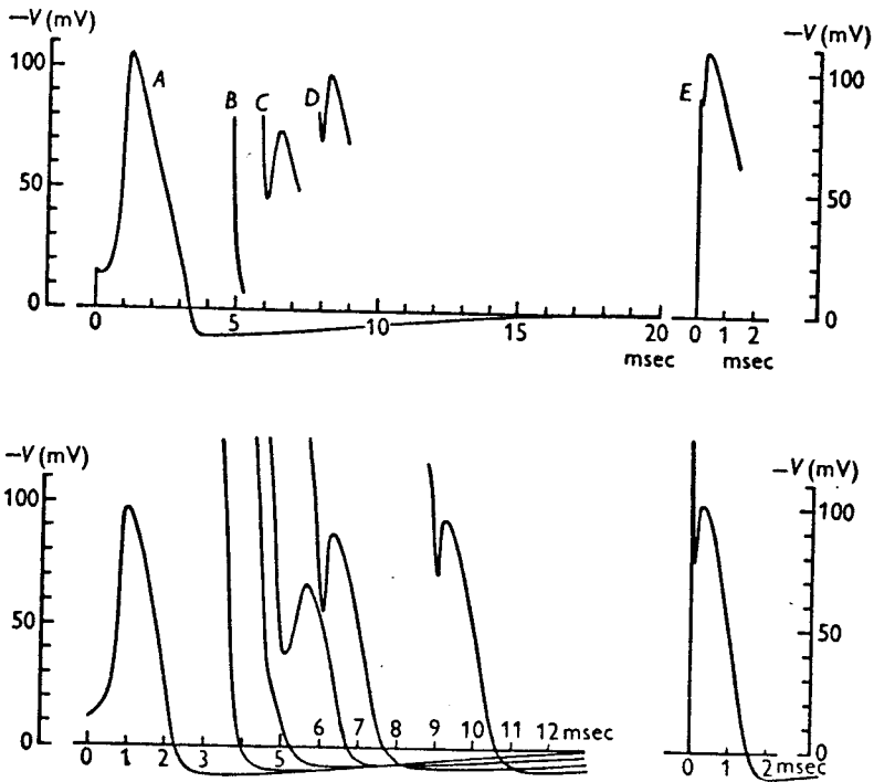
Fig. 20. Theoretical basis of refractory period. Upper curves: numerical solutions of eqn. (26) for temperature of 6° C. Curve A gives the response to 15 \mu\text{coulomb}/\text{cm}^2 applied instantaneously at t=0 . Curve E gives the response to 90 \mu\text{coulomb}/\text{cm}^2 again applied in the resting state. Curves B to D show effect of applying 90 \mu\text{coulomb}/\text{cm}^2 at various times after curve A . Lower curves: a similar experiment with an actual nerve, temperature 9° C. The voltage scales are the same throughout. The time scales differ by a factor appropriate to the temperature difference.
