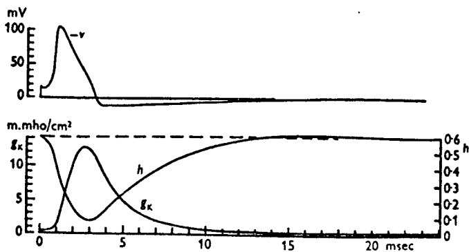
Fig. 19. Numerical solution of eqn. (26) for initial depolarization of 15 mV and temperature of 6° C. Upper curve: membrane potential, as in Fig. 13. Lower curves show time course of g_K and h during action potential and refractory period.
