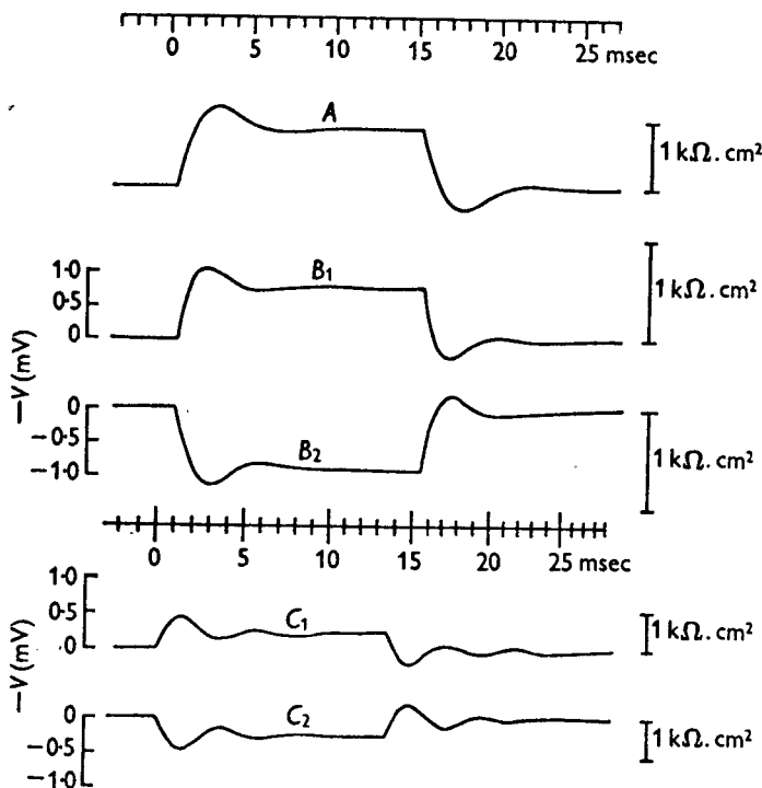
Fig. 23. A , solution of eqn. (35) for small constant current pulse; temperature 18.5^{\circ}\text{C} ; linear approximation. The curve shows \delta V/\delta I (plotted upwards) as a function of time. B , changes in membrane potential associated with application of weak constant currents of duration 15 msec and strength \pm 1.49 \mu\text{A}/\text{cm}^2 . B 1 , cathodic current; B 2 , anodic current. Depolarization is shown upward. Temperature 19^{\circ}\text{C} . C , similar records from another fibre enlarged to have same time scale. Current strengths are \pm 0.55 \mu\text{A}/\text{cm}^2 . Temperature 18^{\circ}\text{C} . The response is unusually oscillatory.
