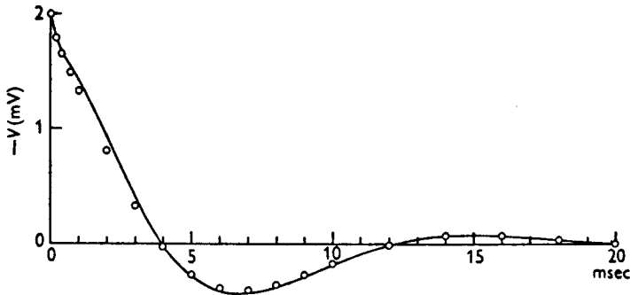
Fig. 24. Comparison of step-by-step solution and linear approximation. Eqn. (26), temperature 6° C; initial displacement of -V = 2 mV. Continuous line: step-by-step solution. Circles: linear approximation with same initial displacement.
