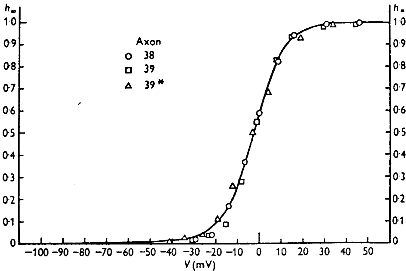
Fig. 10. Steady state relation between h and V . The smooth curve is drawn according to eqn. (25). The experimental points are those given in Table 1 of Hodgkin & Huxley (1952 c ). Axon 38 (5° C) as measured. Axon 39 (19° C) displaced -1.5 mV. Axon 39* (3° C, fibre in derelict state) displaced -12 mV. The curve gives the fraction of the sodium-carrying system which is readily available, as a function of membrane potential, in the steady state.
