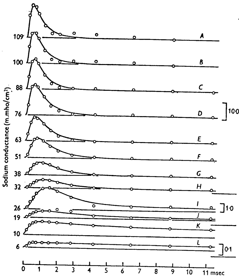
Fig. 6. Changes of sodium conductance associated with different depolarizations. The circles are experimental estimates of sodium conductance obtained on axon 17, temperature 6–7° C (cf. Fig. 3). The smooth curves are theoretical curves with parameters shown in Table 2; A to H drawn from eqn. 19, I to L from 14, 17, 18 with \bar{g}_{Na} = 70.7 m.mho/cm 2 . The ordinate scales on the right are given in m.mho/cm 2 . The numbers on the left show the depolarization in mV. The time scale applies to all curves.
